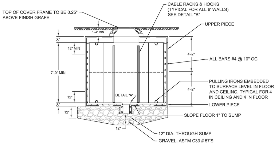
ELEVATION NTS
