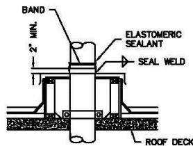
DETAIL - THIMBLE
