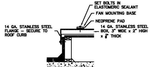
DETAIL - EQUIPMENT MOUNTING RAIL
