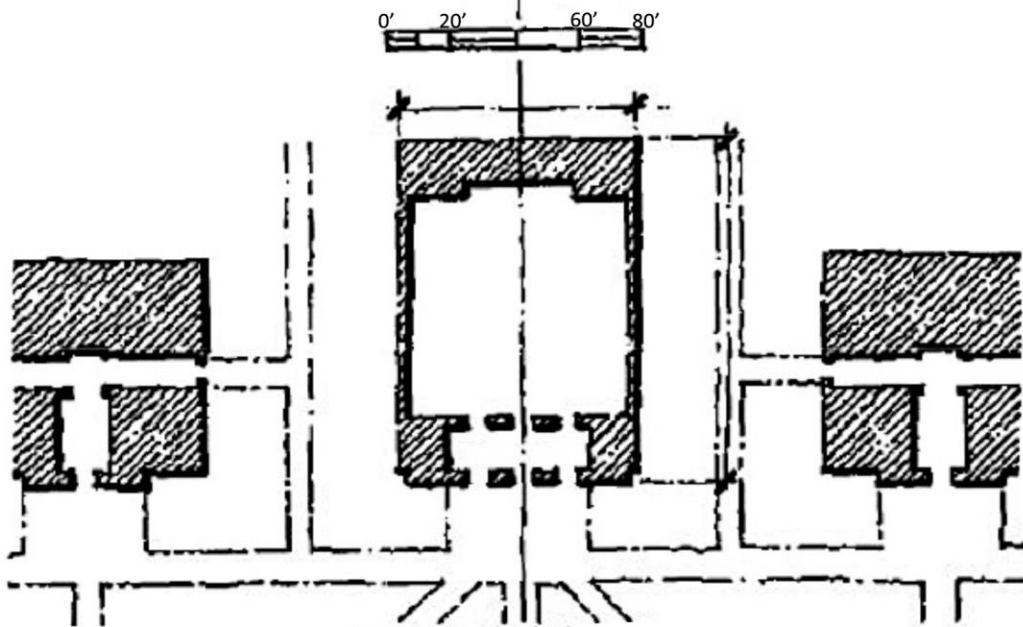
Typical Plan
