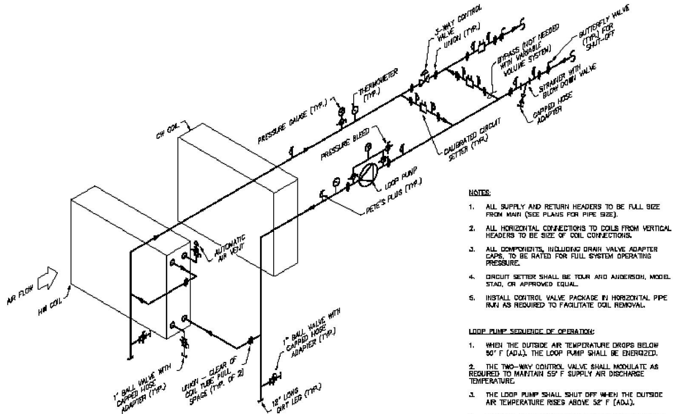
A.H.U. COIL PIPING DETAIL – HOT WATER COIL WITH LOOP PUMP & 2-WAY VALVE
