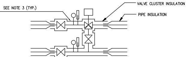
INSULATION TIE DOWN AT EQUIPMENT COLD PIPING
