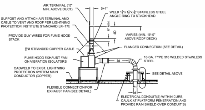
TYPICAL DETAIL - FUME HOOD EXHAUST FAN SUPPORT FRAME SCALE: NONE
