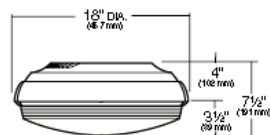
Fixture with Standard Acrylic Refractor
