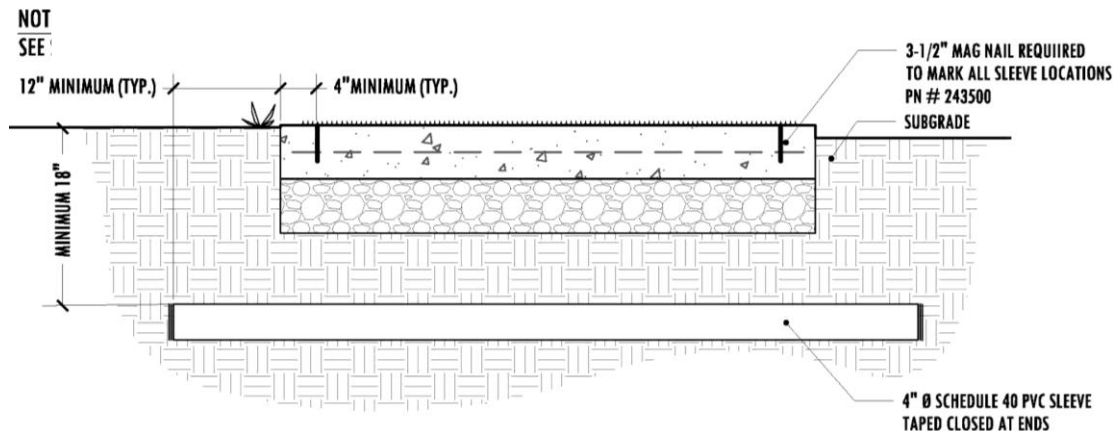
Sleeving Detail
